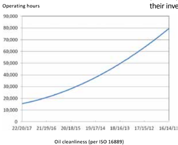
Figure 2: Projected engine life, with oil analysis.
